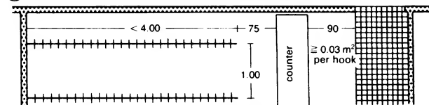
⑥ Supervised cloakroom, single rows of hooks
